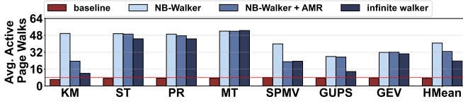
Fig. 13: Average number of concurrent page table walks.
