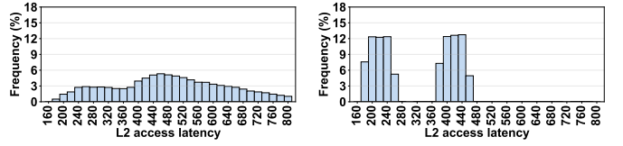
(a) FWT (low-MPKI)
