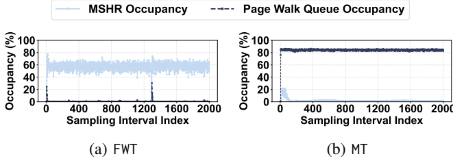
Fig. 9: Dynamic resource occupancy of L1 MSHRs vs. PWQs. Sampling over 1,000-cycle intervals.
