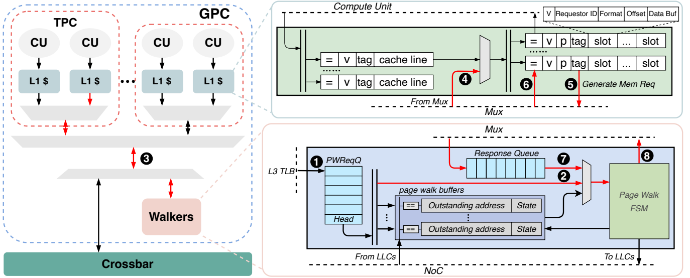
Fig. 10: Schematic overview of the NB-WALKER non-blocking page table walk subsystem.
