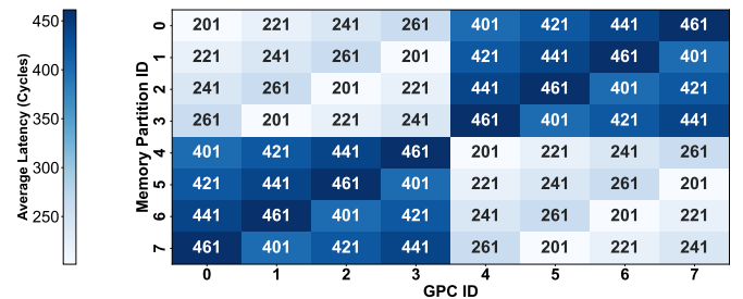
Fig. 11: Non-uniform L2 hit latency in our baseline [8].
