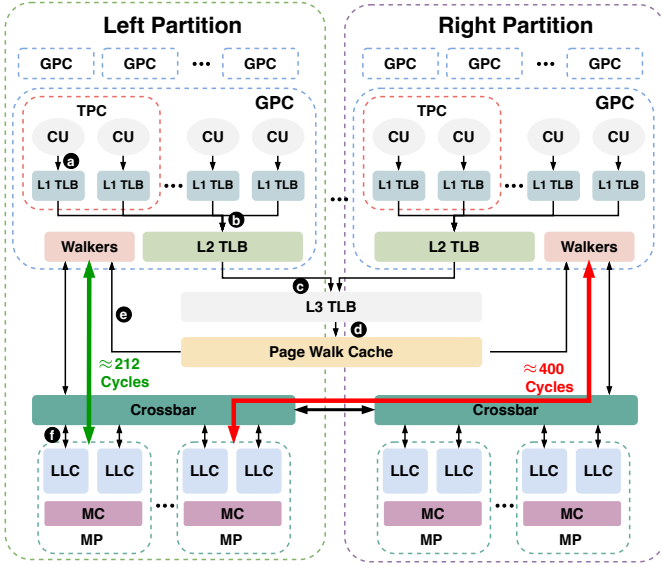
Fig. 1: TLB structure and address translation process in modern GPUs [8], [19]–[21]. Walkers follow a blocking design that keeps them occupied until each walk completes, while PTW memory accesses suffer from non-uniform latency due to internal NUMA effects.
