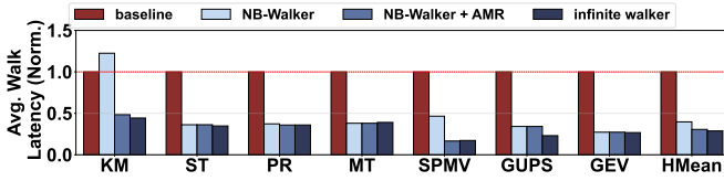
Fig. 14: Normalized page table walk latency.
