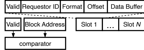
Fig. 3: Overview of an explicitly addressed MSHR entry.
