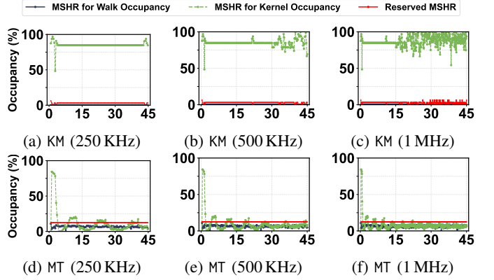
Fig. 24: Impact of profiling frequency on time-series MSHR utilization and AMR reservations for KM (top row) and MT (bottom row). The x-axis is measured in cycles ( \times 10^4 ).
