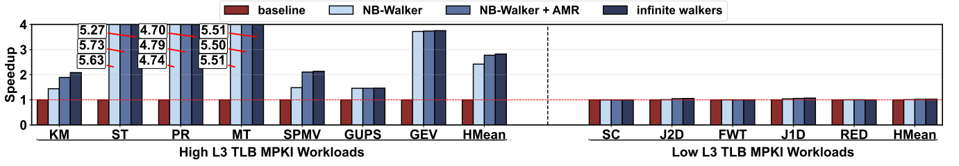
Fig. 12: Speedup of NB-WALKER, NB-WALKER+AMR, and an idealized configuration with infinite walkers.
