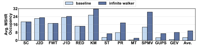
Fig. 8: Average L1 MSHR occupancy across different benchmarks under baseline GPU and idealized configuration with infinite walkers.
