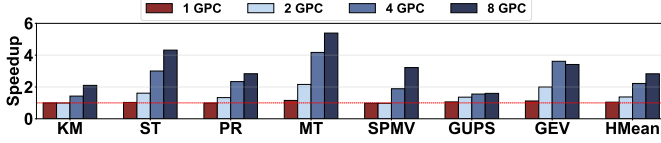
Fig. 18: Speedup of NB-WALKER+AMR over the baseline GPU with varying numbers of GPCs (1, 2, 4 and 8).
