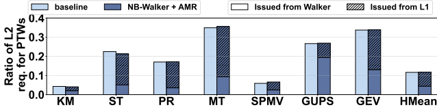
Fig. 17: Fraction of L2 access requests issued for servicing page table walks in the baseline and NB-WALKER+AMR.
