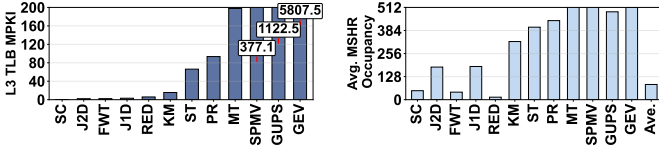
Fig. 4: L3 TLB MPKI (left) and Average L3 TLB MSHR occupancy (right) on the baseline GPU .
