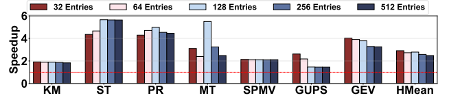
Fig. 19: Speedup of NB-WALKER+AMR over the baseline GPU with varying PWC entries.
