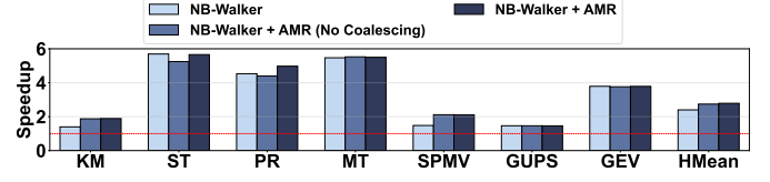
Fig. 16: Speedup over the baseline GPU for NB-WALKER, NB-WALKER+AMR (without L1 MSHR PTE coalescing) and NB-WALKER+AMR.
