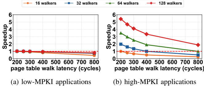
Fig. 7: Performance speedup for (a) low-MPKI and (b) high-MPKI applications across varying page table walker counts and walk latencies, normalized to a baseline with 16 walkers and a 200-cycle walk latency.
