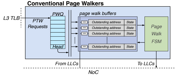
Fig. 2: Overview of page walkers in the baseline GPU.
