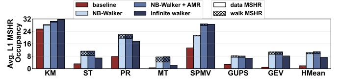
Fig. 15: Breakdown of average L1 MSHR occupancy.
