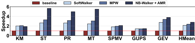
Fig. 25: Performance comparison between NB-WALKER, Marching Page Walks (MPW) [16] and SOFTWALKER [23], normalized to the baseline GPU.
