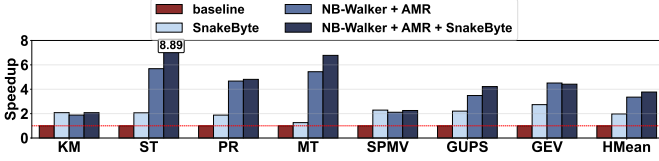
Fig. 26: Performance comparison between NB-WALKER and SNAKEBYTE [49], normalized to the baseline GPU.
