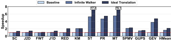
Fig. 5: Performance speedup for baseline GPU, infinite page walkers, and ideal translation configuration.
