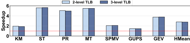
Fig. 22: Speedup of NB-WALKER+AMR over the baseline GPU under two-level and three-level TLB hierarchies.
