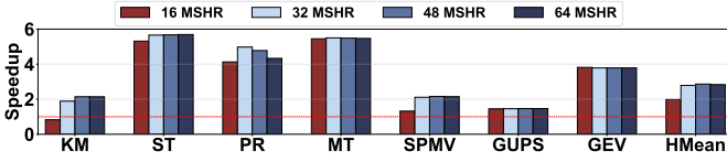
Fig. 21: Speedup of NB-WALKER+AMR over the baseline GPU with varying L1 MSHR capacity (16, 32, 48, 64 entries).
