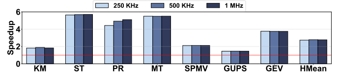
Fig. 23: Speedup of NB-WALKER+AMR over the baseline GPU with varying profiling frequency.
